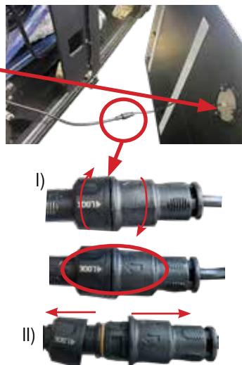
4 Disconnect logo light wire from back side of door panel
